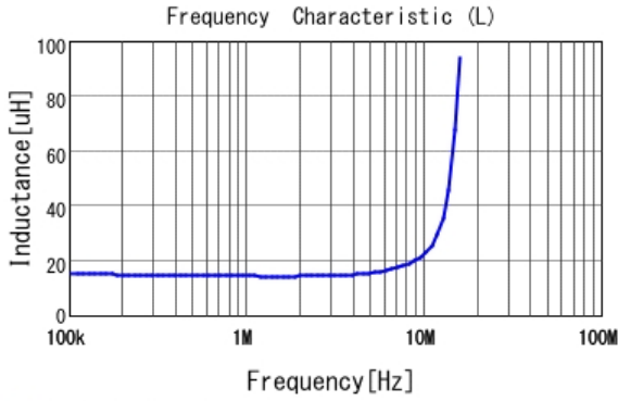
■ LQH5BPN150M38 L
