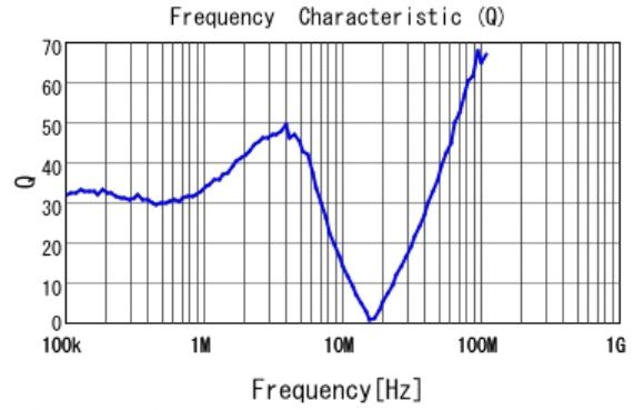
■ LQH5BPN150M38 Q
