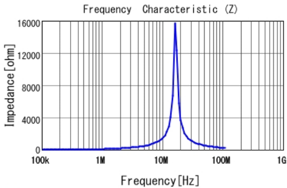
■ LQH5BPN150M38 |Z|
