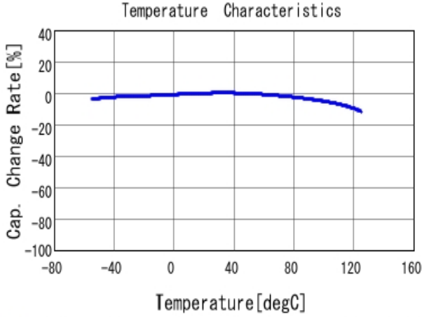
■ GCJ188R71E105KA01 C-Temp. capchange, DC0.0V, AC1.0V rm
