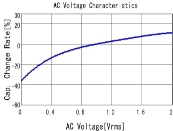
■ GCJ188R71E105KA01 C-AC Voltage capchange, DCOV, 25.0d
