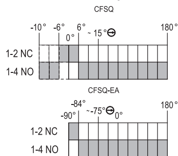
Stroke diagram
