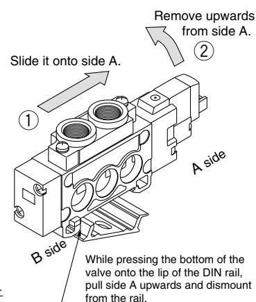
Fig. 2 Manifold dismounting procedure
