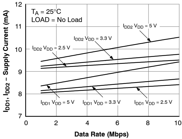
Figure 5. NCID9411 Supply Current vs. Data Rate (No Load)
