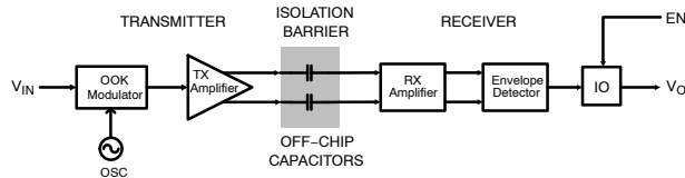
Figure 17. Operational Block Diagram of Single Channel
