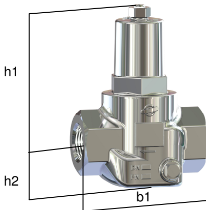
DN 15 - DN 32
