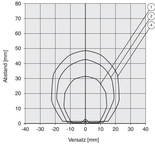
Leseabstand in Luft IPC02-16
