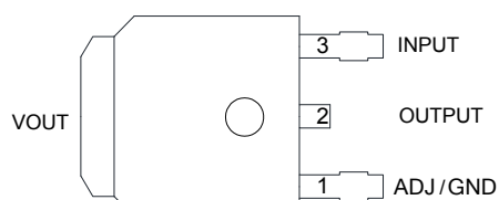
TO252-2 (4)
