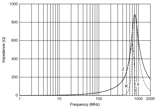
BLM15BA330SN1
