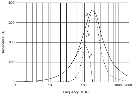
BLM15BD102SN1
