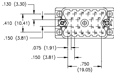
20 PIN PLUG
