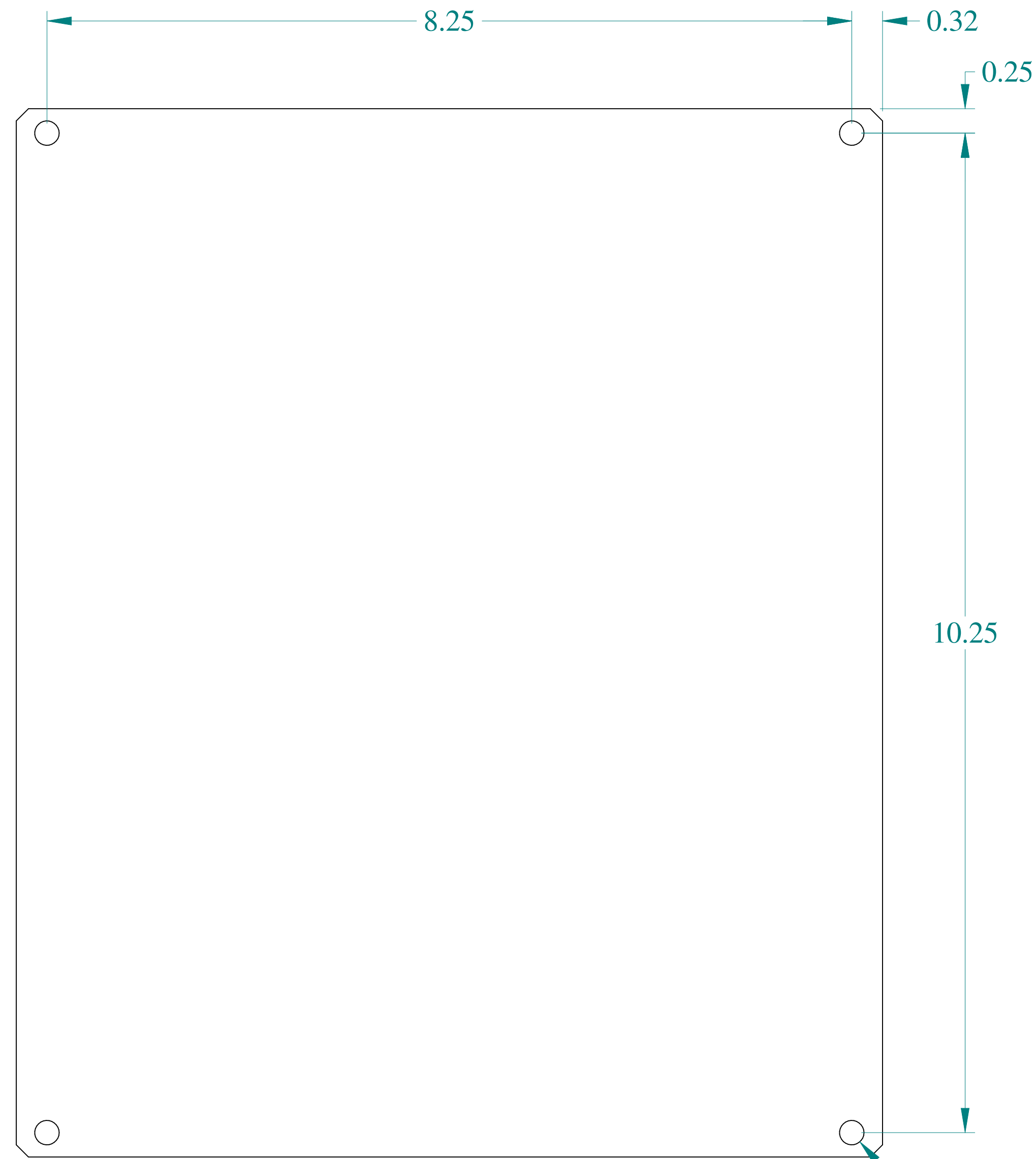
FRONT VIEW
