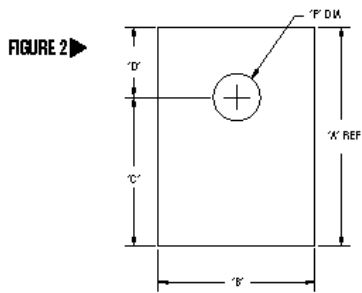
Mica Insulator for TO-220 device
