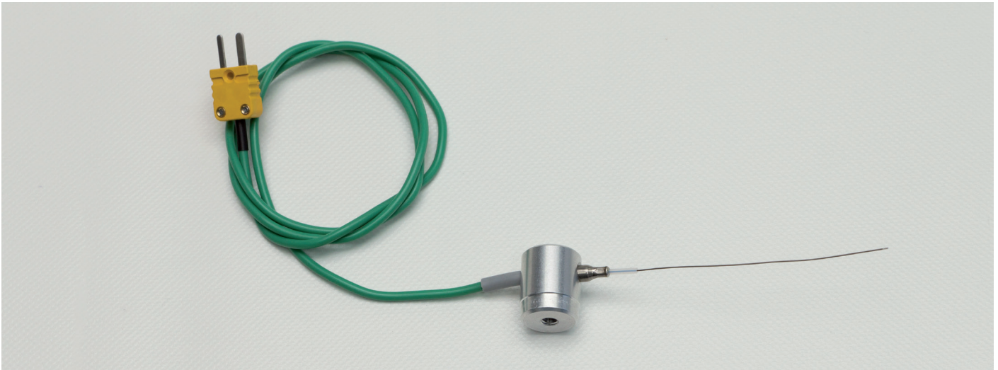
Abbildung/Figure 1: Thermoelement AccuTC / AccuTC thermocouple
