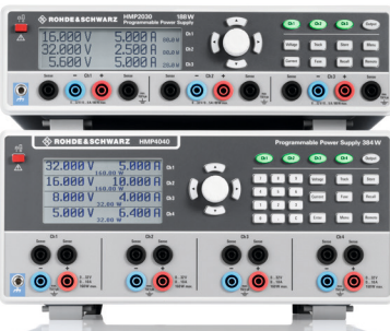
R&S®HMP2030 three-channel and R&S®HMP4040 four-channel power supply
