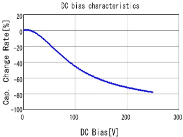
■ KRM55TR72E225MH01 C-DC bias capchange, 25.0degC, AC1V
