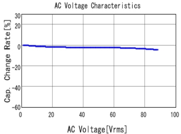
■ KRM55TR72E225MH01 C-AC Voltage capchange, DCOV, 25.0d
