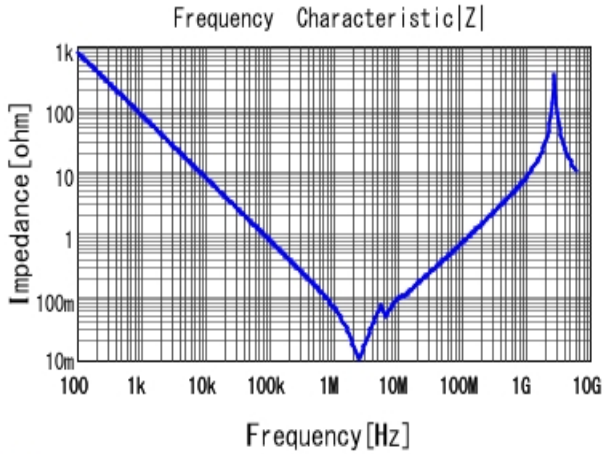
■ KRM55TR72E225MH01 |Z| DCOV, 25degC
