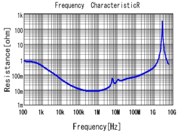
■ KRM55TR72E225MH01 R DCOV, 25degC
