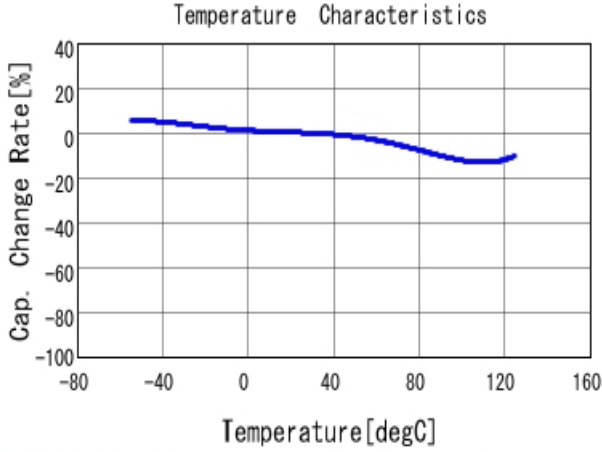
■ KRM55TR72E225MH01 C-Temp. capchange, DCOV, AC1Vrms
