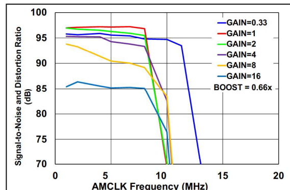
FIGURE 2-36: SINAD vs. AMCLK (Boost = 0.66x , External V_{REF} ).
