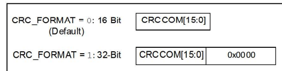
FIGURE 6-10: CRC Format Table for Read Communications.
