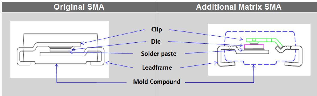
Figure 1: Comparison of Package Construction for GPP Rectifiers and Unidirectional TVS products
