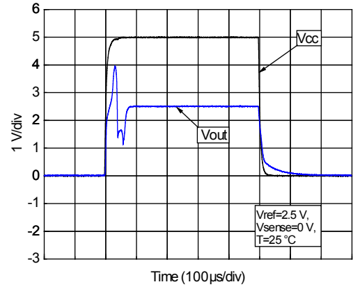
Figure 26. Start-up response
