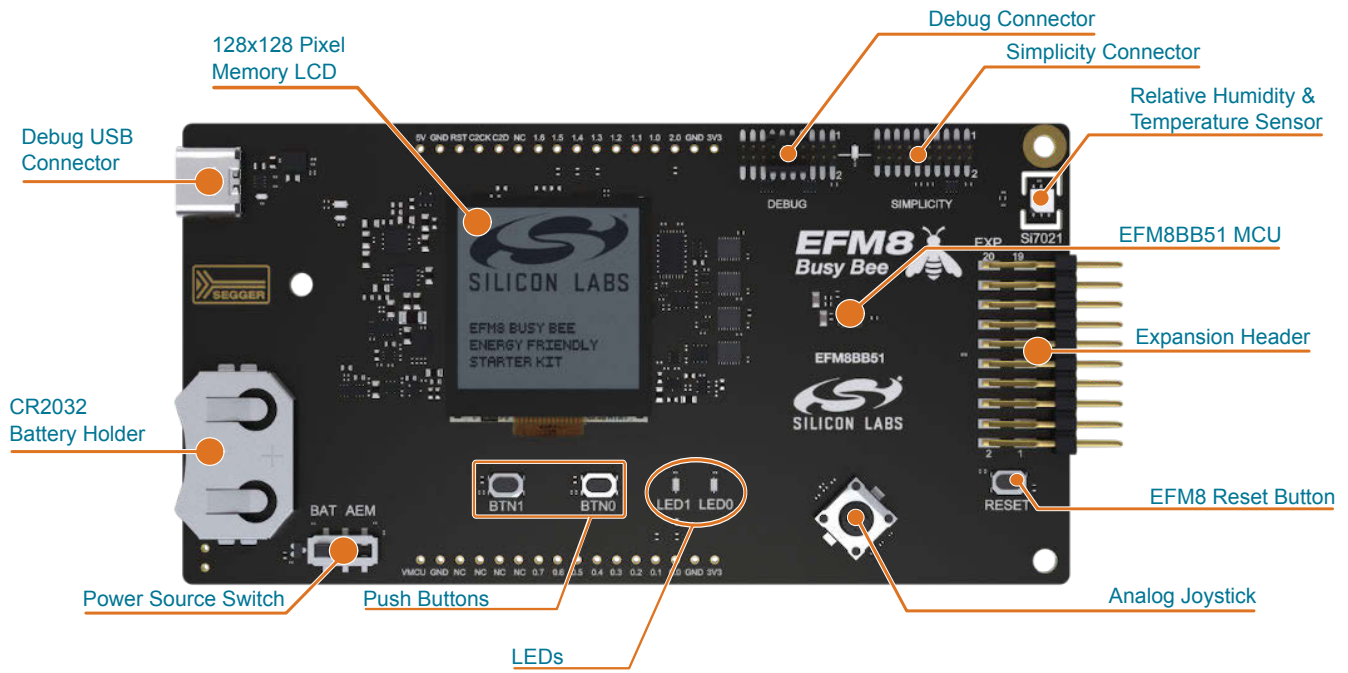
Figure 3.1. BB51 Pro Kit Hardware Layout
