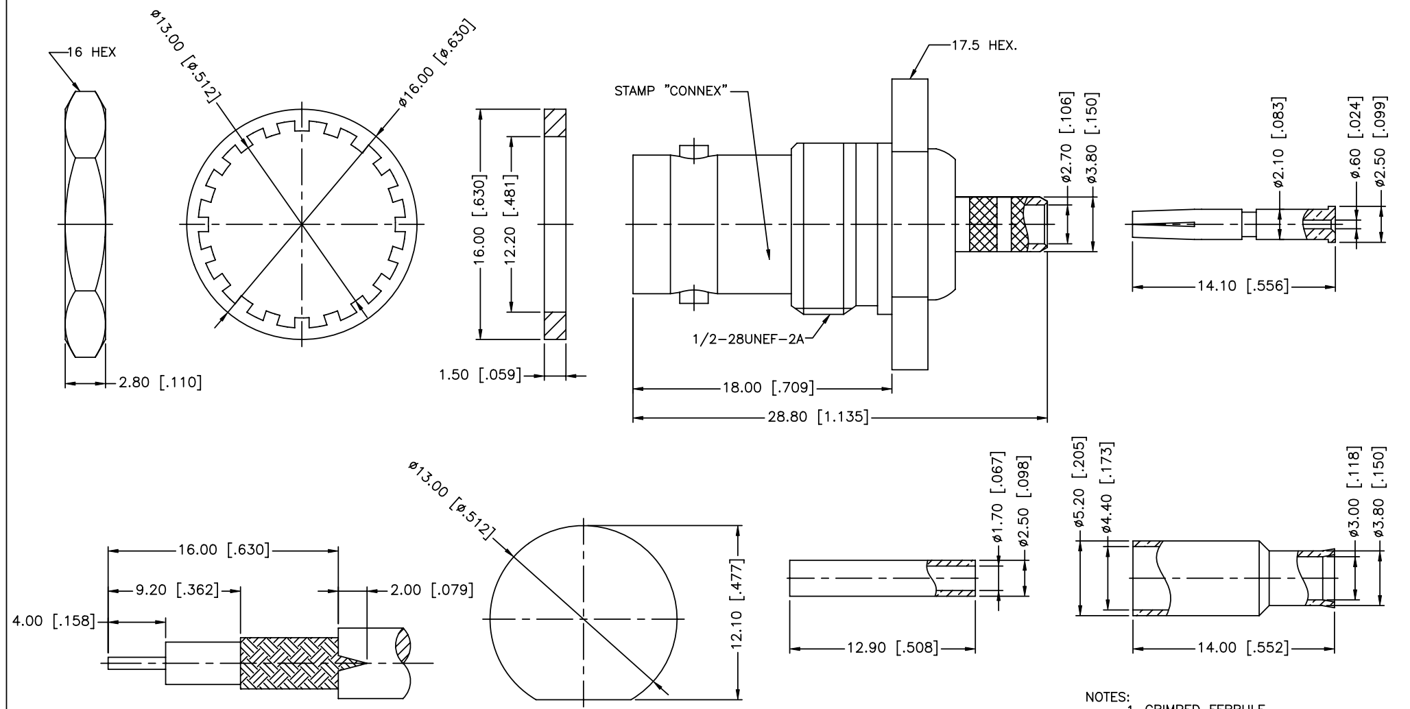
RECOMMENDED CABLE STRIPPING DIM'S
