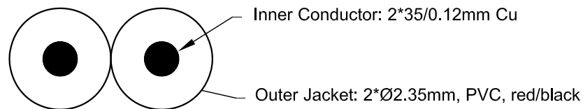
Cable Structure
