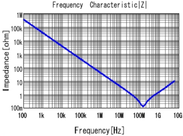
■ GRM033R61E472KA12 |Z| DCOV, 25degC
