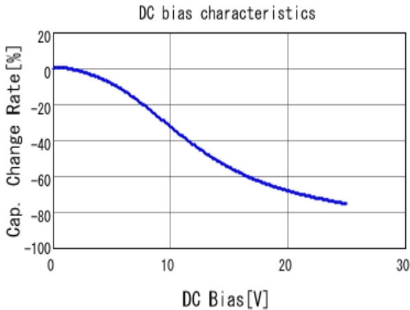
■ GRM033R61E472KA12 C-DC bias capchange, 25.0degC, AC1.
