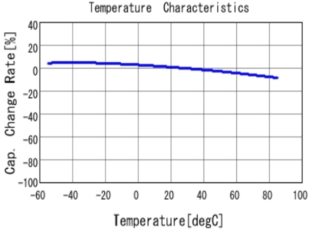
■ GRM033R61E472KA12 C-Temp. capchange, DCO. 0V, AC1.0Vrm
