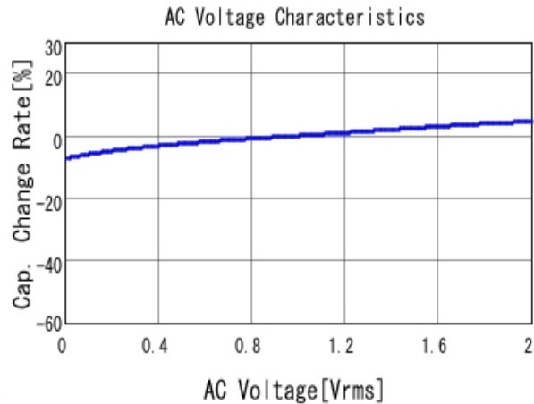
■ GRM033R61E472KA12 C-AC Voltage capchange, DCOV, 25.0d
