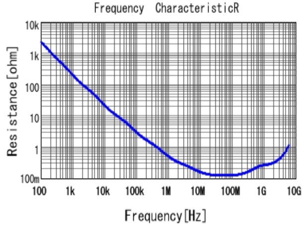
■ GRM033R61E472KA12 R DCOV, 25degC
