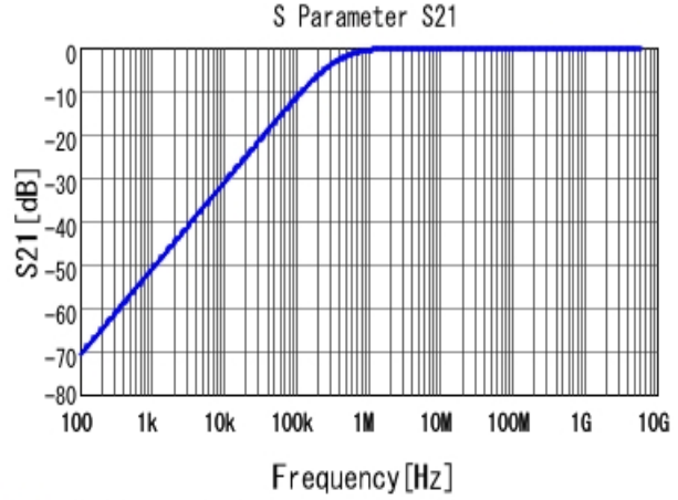
■ GRM033R61E472KA12 S21 DCOV, 25degC
