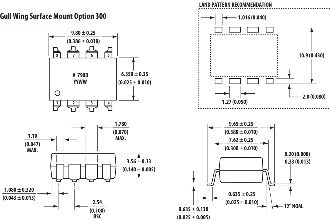
Figure 2. Gull Wing Surface Mount Option 300
