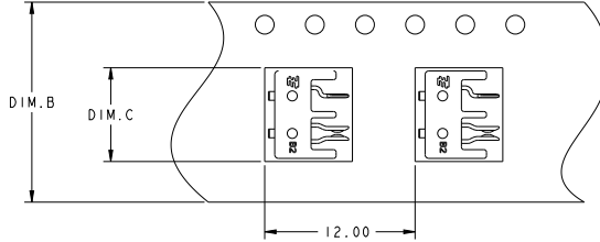
2, 4 and 6 position showing 2 mated parts
