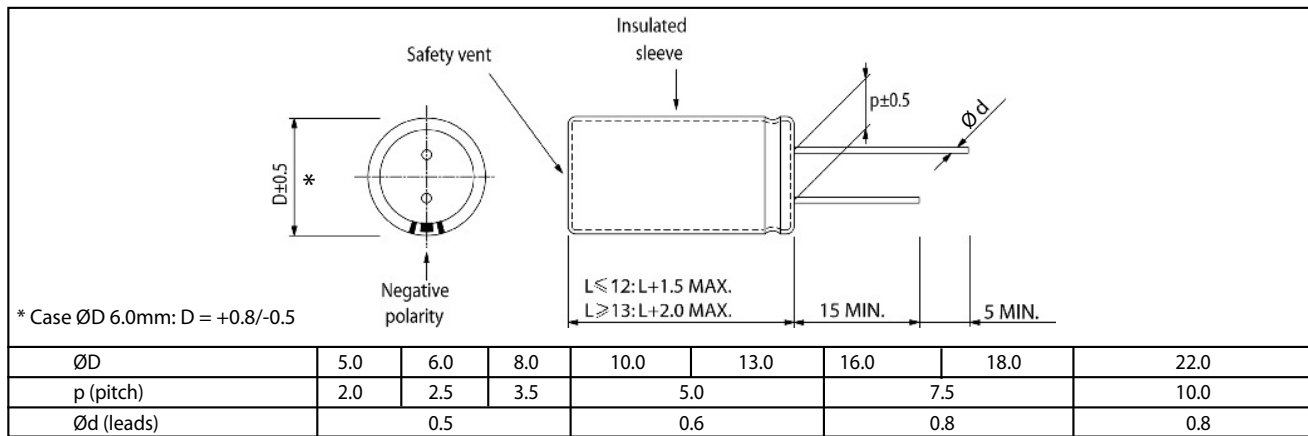
Diagram of dimensions (Units=mm)
