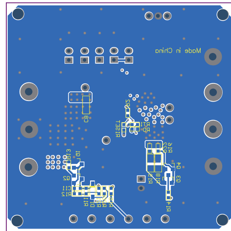
Figure 14: Bottom Layer
