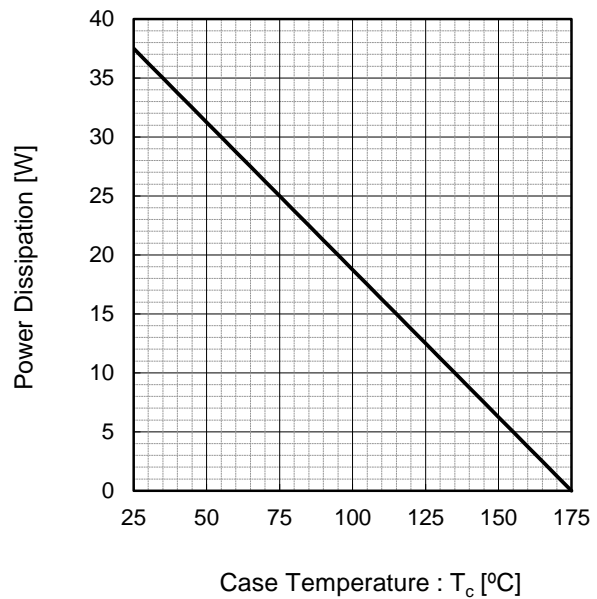
Fig.6 Power Dissipation
