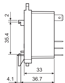
066.07 with relay
