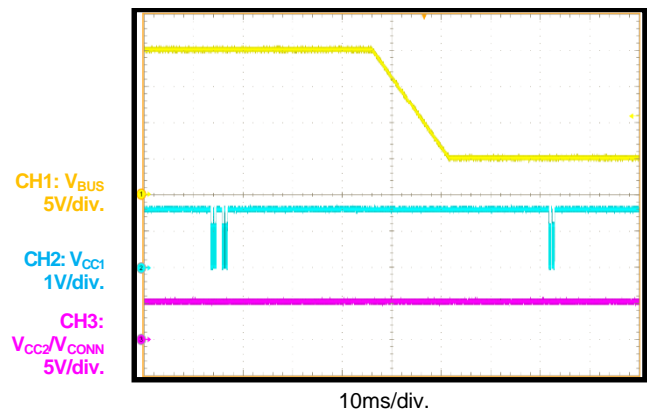
PDO Transition 20V PDO to 5V PDO
