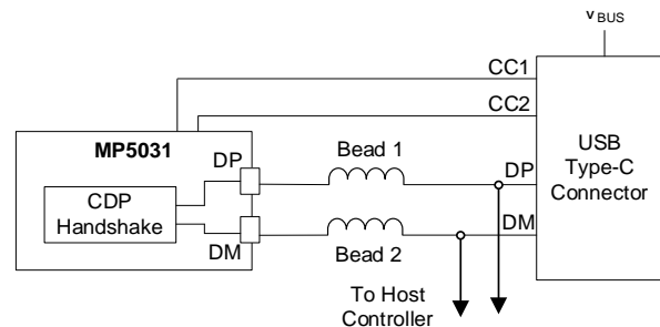
Figure 17: CDP Mode Set-Up
