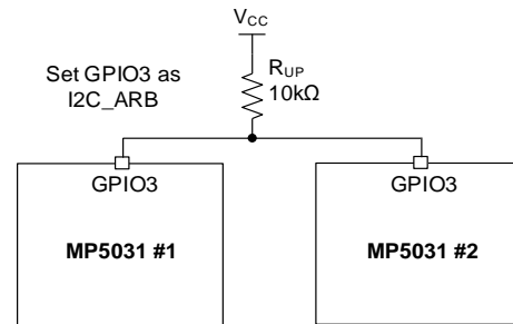
Figure 16: I 2 C Arbitration Connection
