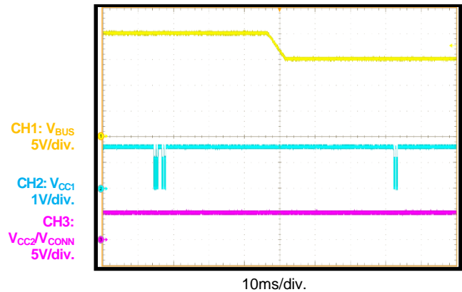
PDO Transition 20V PDO to 15V PDO
