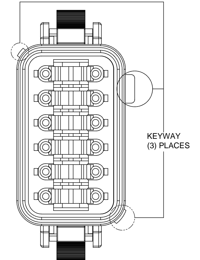
P/N AT06-12SD KEY-D CONFIGURATION STANDARD COLOR: BROWN
