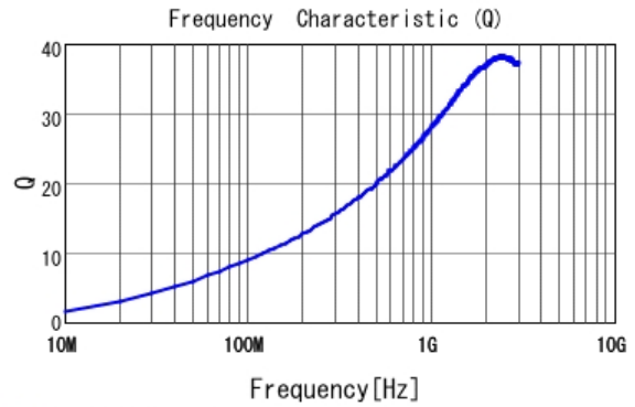
■ LQP03TN5N6J02 Q
