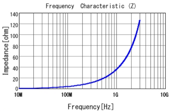
■ LQP03TN5N6J02 |Z|
