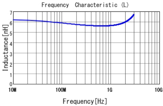
■ LQP03TN5N6J02 L
