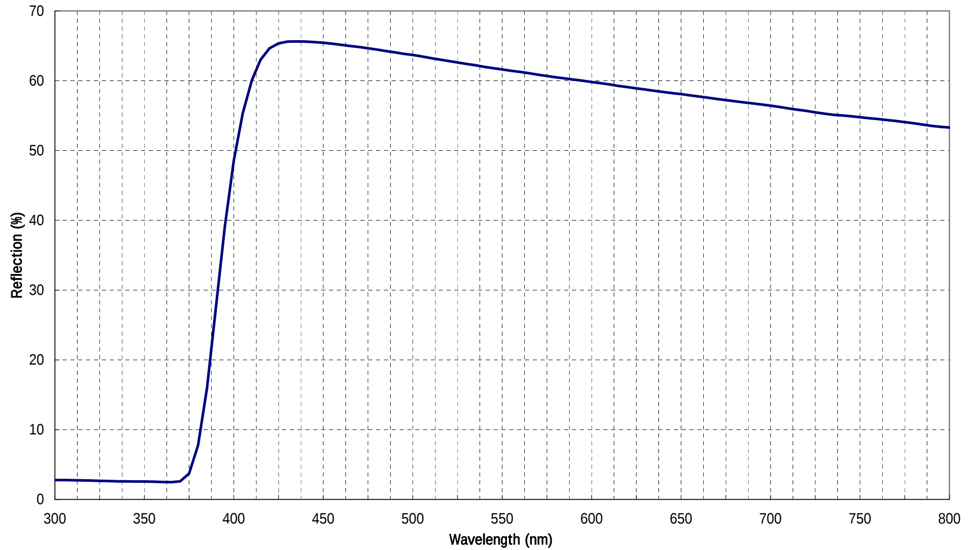
CLAREX LightGuide Reflector DR-IIA 705B
