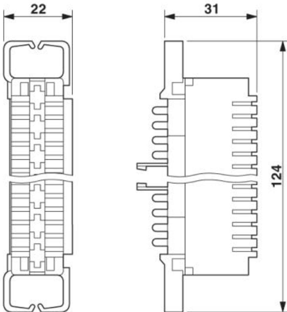
Dimensional drawing
