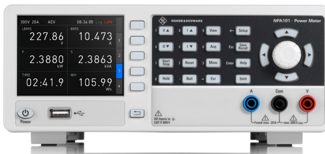
R&S®NPA101
