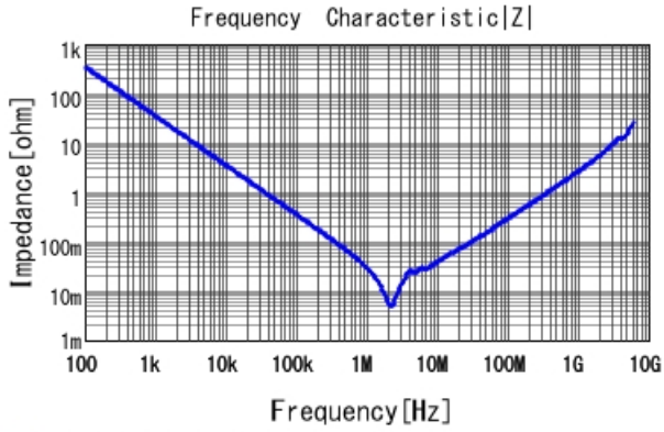
■ GRM31CR71H475KA12 |Z| DCOV, 25degC
