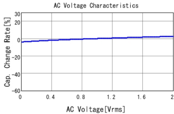
■ GRM31CR71H475KA12 C-AC Voltage capchange, DCOV, 25.0d
