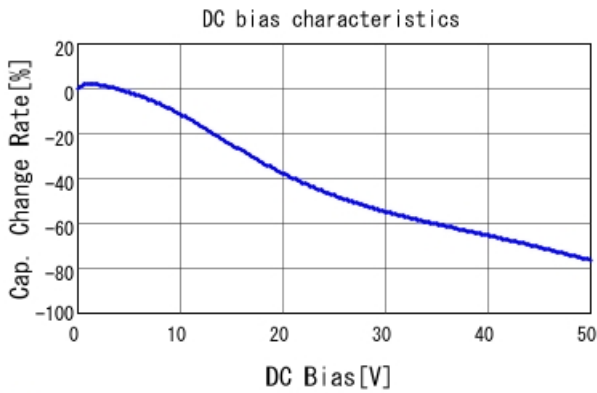
■ GRM31CR71H475KA12 C-DC bias capchange, 25.0degC, AC1.
