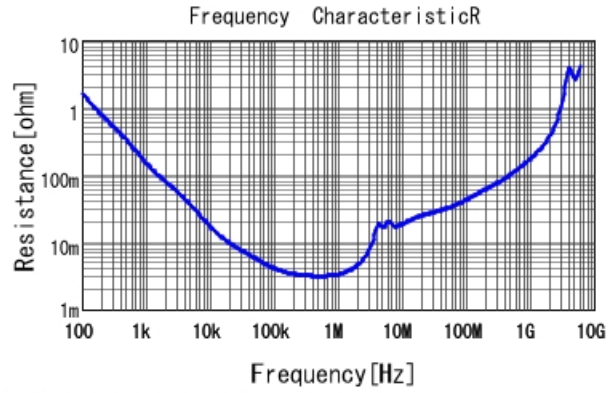
■ GRM31CR71H475KA12 R DCOV, 25degC
