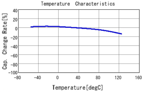
■ GRM31CR71H475KA12 C-Temp. capchange, DCO. 0V, AC1. 0Vrm
