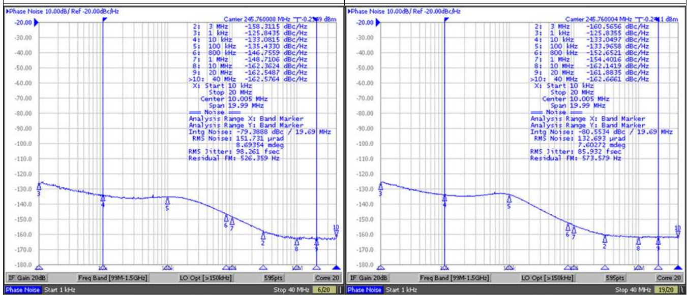
VCO_MUX = 0 (VCO0) PLL2 Loop Filter Bandwidth = 303 kHz VCO0 = 1966.08 MHz PLL2 Phase Margin = 73° DCLKout2_DIV = 8 Figure 4. LMK04826 DCLKout2 Phase Noise
