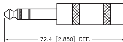
ASSEMBLY
