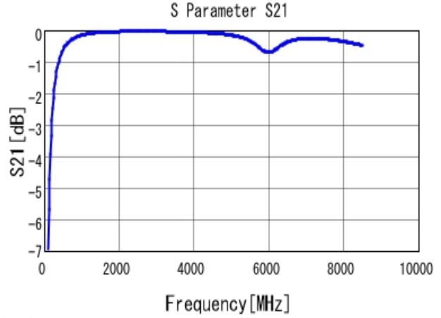
■ GCM1555C1H8R0BA16 S21 DCOV, 25degC
