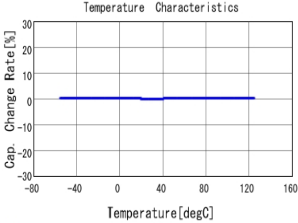
■ GCM1555C1H8R0BA16 C-Temp. capchange, DCOV, AC1Vrms
