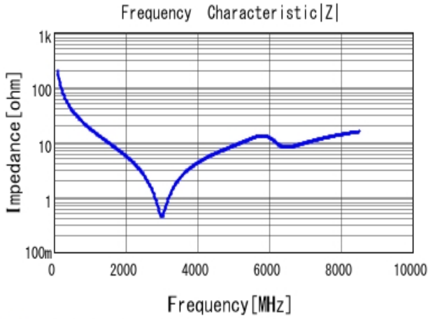
■ GCM1555C1H8R0BA16 |Z| DC0V, 25degC
