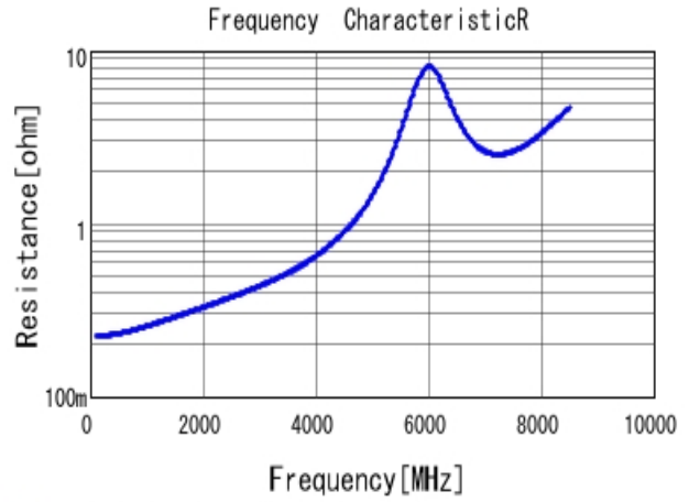
■ GCM1555C1H8R0BA16 R DC0V, 25degC
