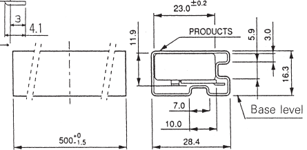
Tube Package Dimensions (Ref.)
