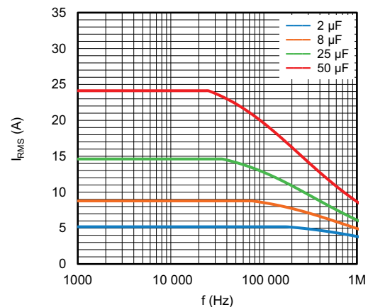
Maximum I_{RMS} vs. frequency for 700 V, ambient temperature of 85 °C (typical curve)
