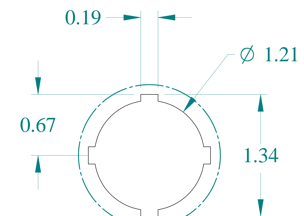
DETAIL Z
