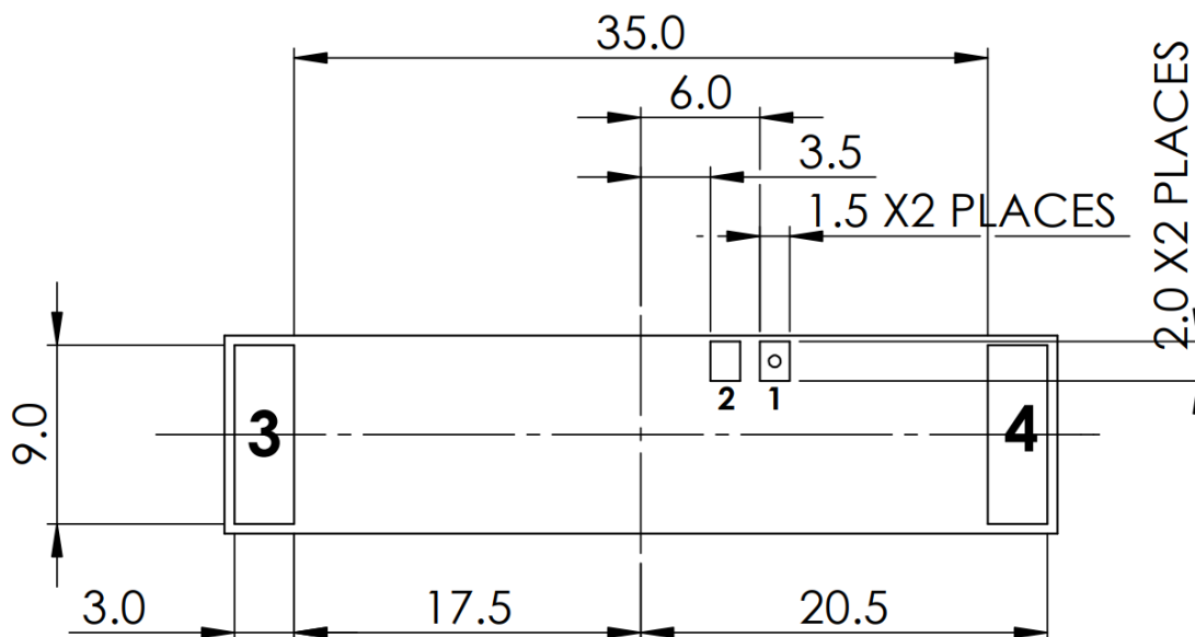
BOTTOM VIEW
