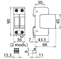
Dimension drawing DG M TT 2P 385 FM
