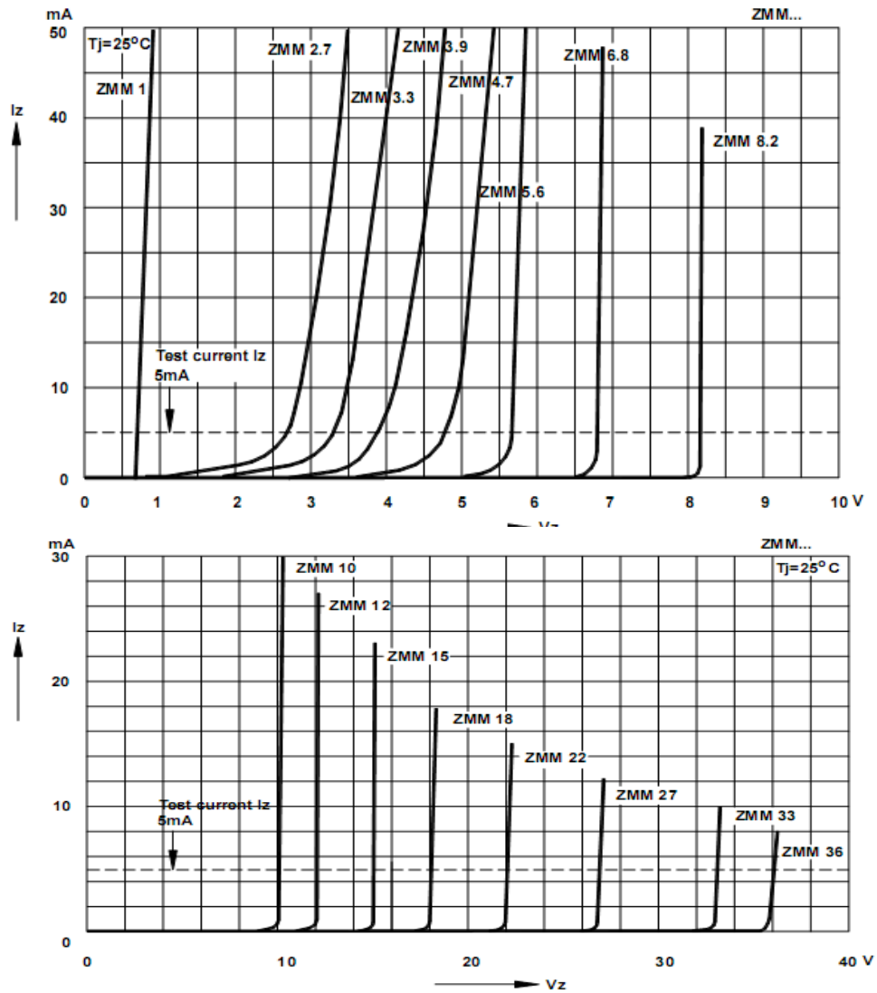
FIG.1- BREAKDOWN CHARACTERISTICS
