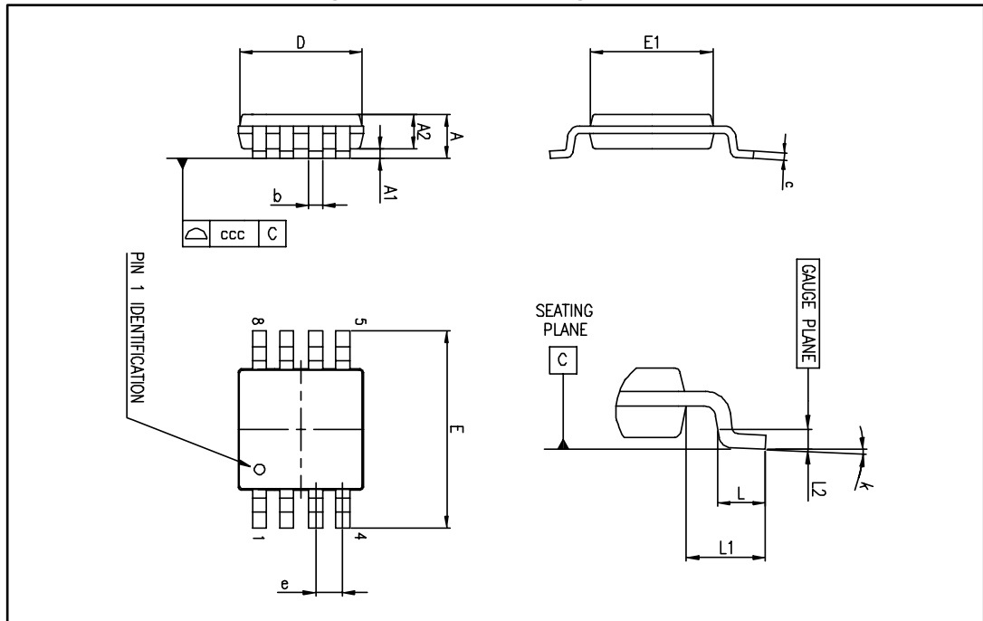
Figure 69: MiniSO8 package outline
