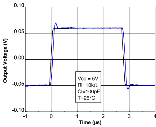
Figure 32: Small signal VCC = 5 V
