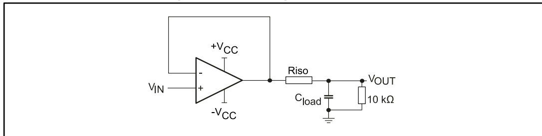
Figure 54: Test configuration for Riso
