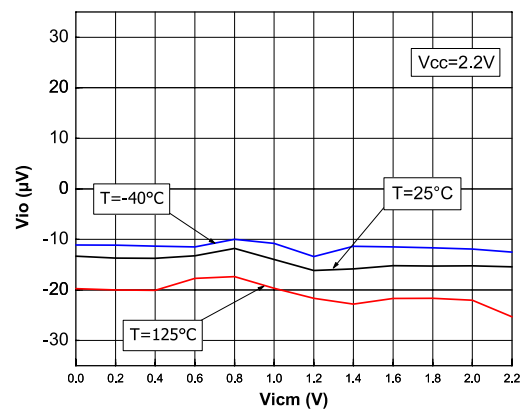
Figure 13: Input offset voltage vs. input common-mode at VCC = 2.2 V
