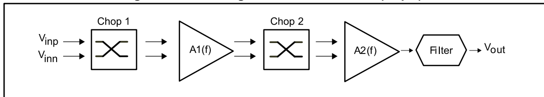
Figure 47: Block diagram in the time domain (step 2)
