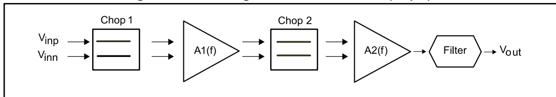
Figure 46: Block diagram in the time domain (step 1)
