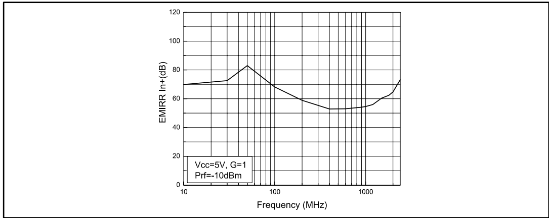
Figure 55: EMIRR on IN+ pin
