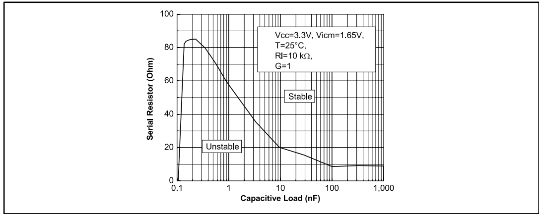
Figure 52: Stability criteria with a serial resistor at VCC = 3.3 V
