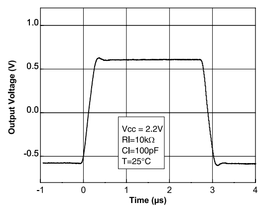
Figure 35: Large signal VCC = 2.2 V
