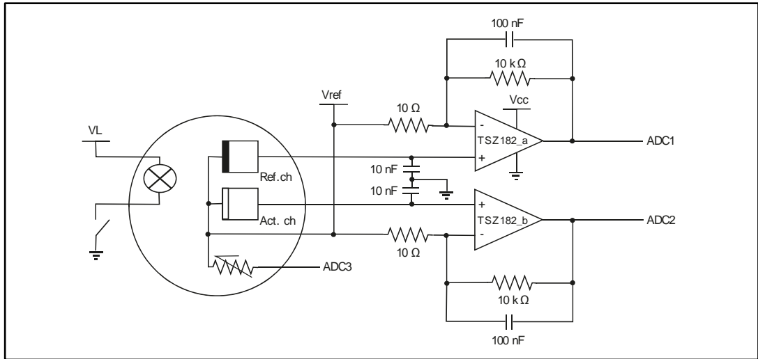
Figure 62: Principle schematic
