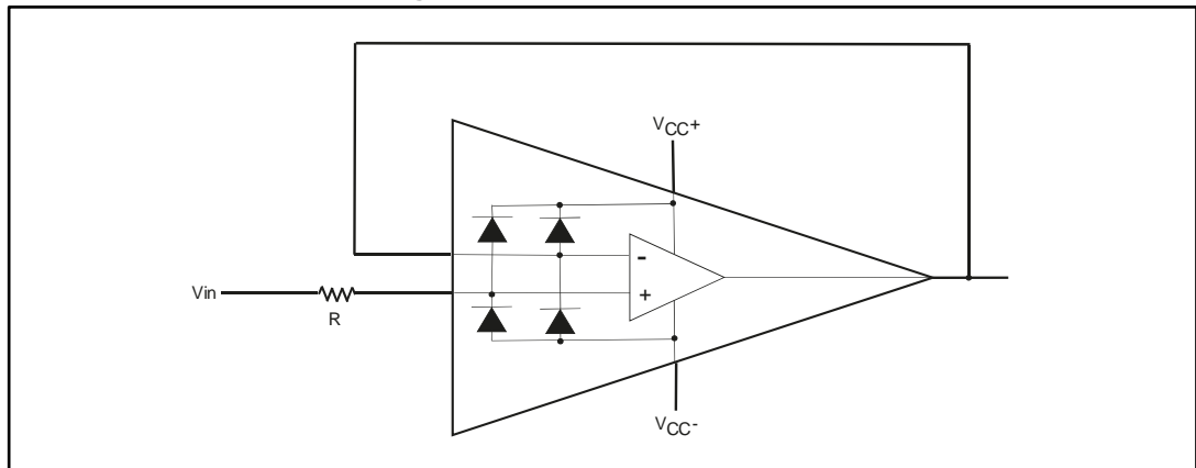
Figure 50: Input current limitation
