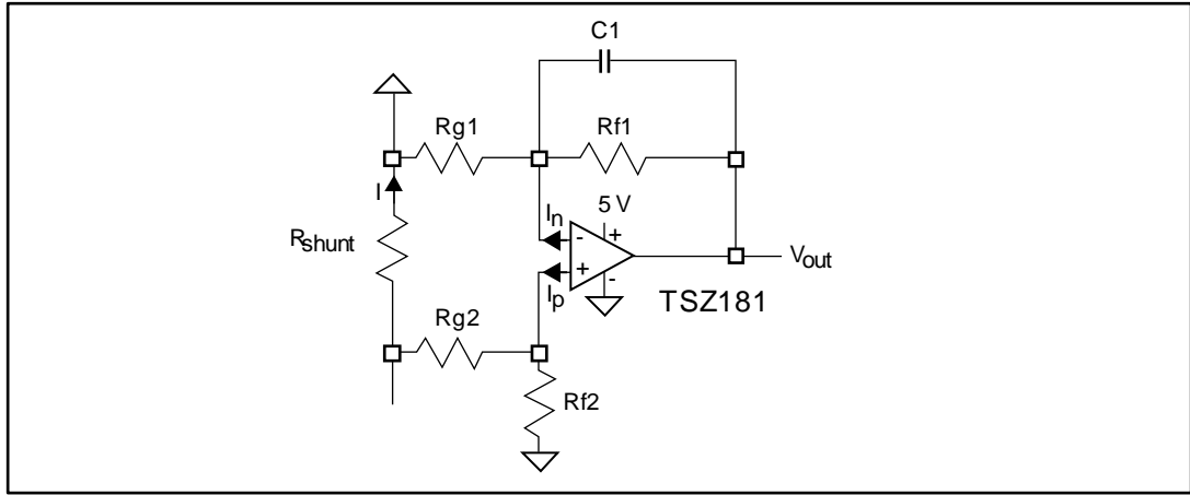
Figure 64: Low-side current sensing schematic
