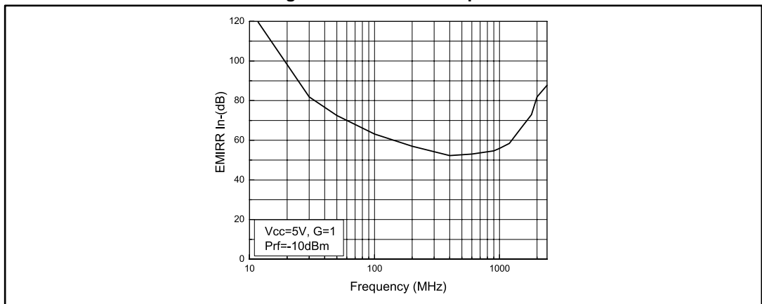
Figure 56: EMIRR on IN- pin
