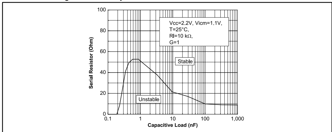
Figure 53: Stability criteria with a serial resistor at VCC = 2.2 V
