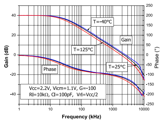
Figure 23: Bode diagram at VCC = 2.2 V
