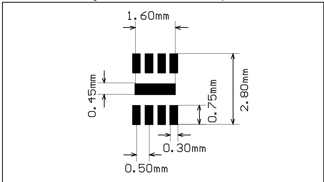
Figure 68: DFN8 2x2 recommended footprint
