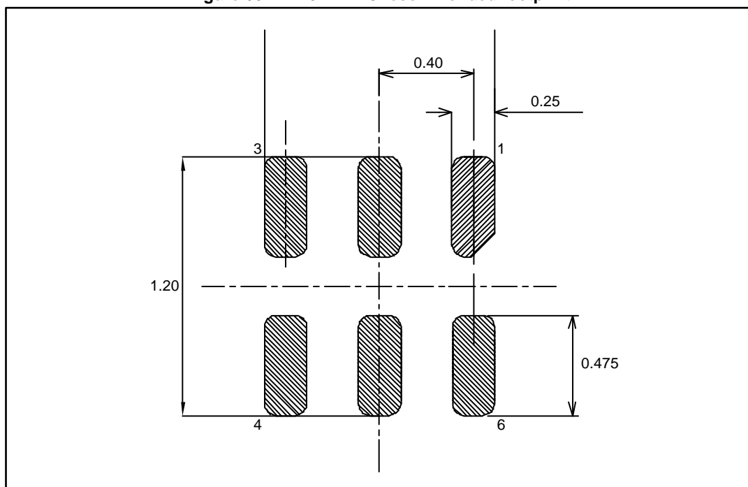
Figure 66: DFN6 1.2x1.3 recommended footprint
