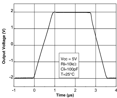
Figure 34: Large signal VCC = 5 V
