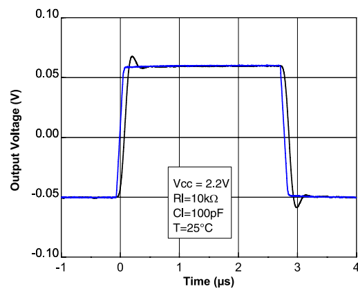
Figure 33: Small signal VCC = 2.2 V
