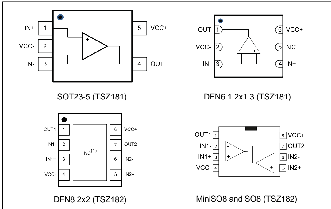
Figure 1: Pin connections for each package (top view)
