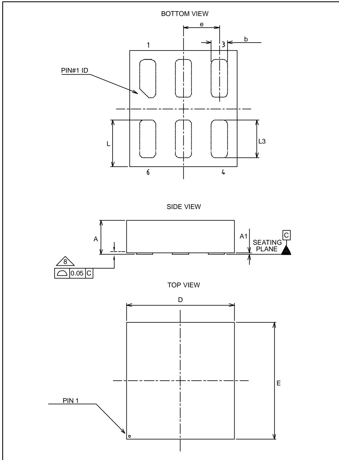
Figure 65: DFN6 1.2x1.3 package outline
