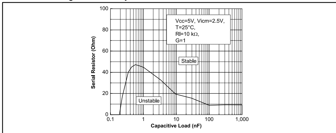
Figure 51: Stability criteria with a serial resistor at VCC = 5 V
