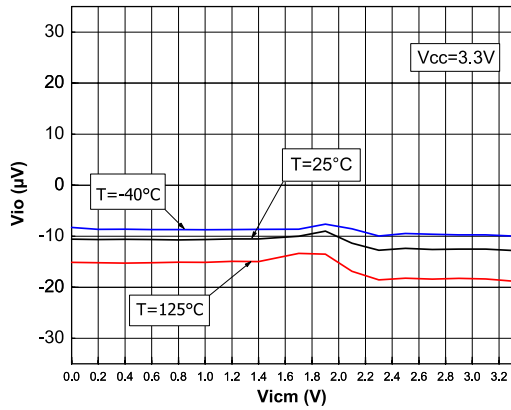
Figure 12: Input offset voltage vs. input common-mode at VCC = 3.3 V
