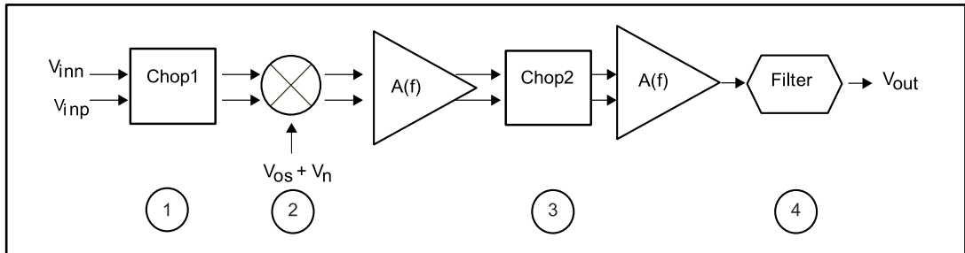
Figure 49: Block diagram in the frequency domain
