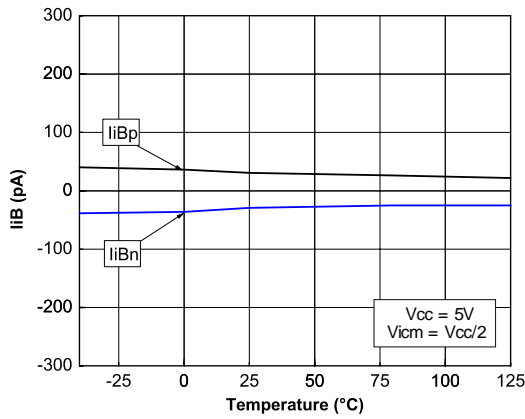
Figure 20: Input bias current vs temperature at VCC = 5 V
