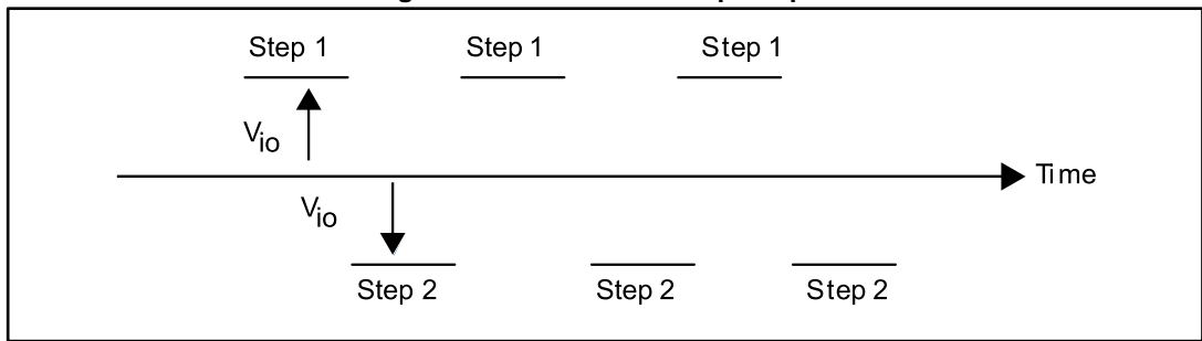
Figure 48: V io cancellation principle
