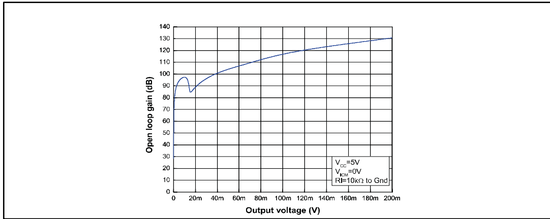
Figure 61: Gain vs. output voltage, VCC = 5 V, RI = 10 kΩ to GND
