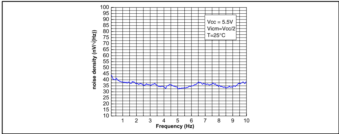
Figure 57: Noise vs frequency between 0.1 and 10 Hz exhibiting no 1/f noise
