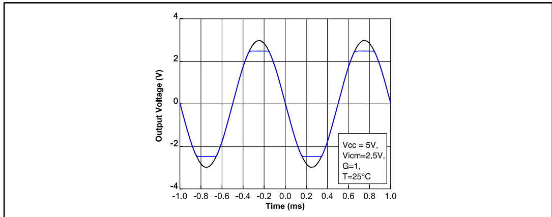
Figure 60: No phase reversal
