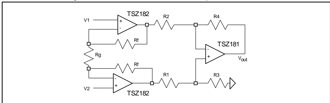
Figure 63: Precision instrumentation amplifier schematic
