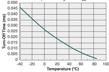
Typical Turn-Off Time vs. Temperature ( I_F=10mA, I_L=50mA_{DC} )
