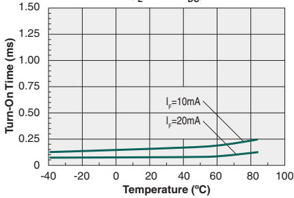
Typical Turn-On Time vs. Temperature ( I_L=50mA_{DC} )
