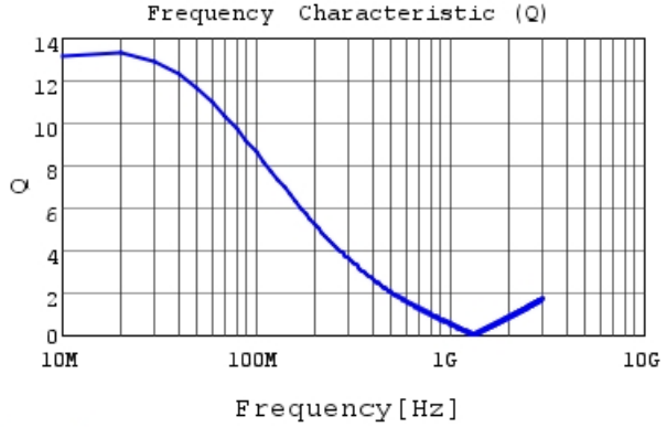
LQW18CNR27J0H Q
