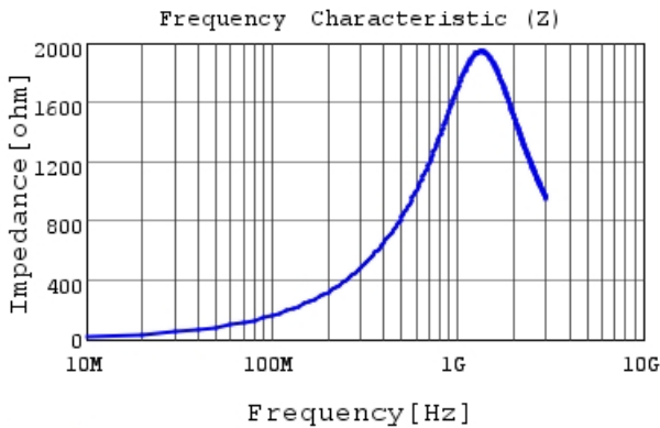
LQW18CNR27J0H |Z|
