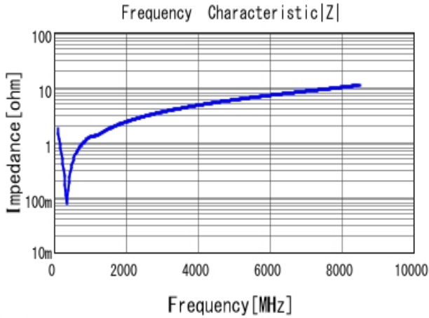
■ GRM0335C1E821JA01 |Z| DCOV, 25degC
