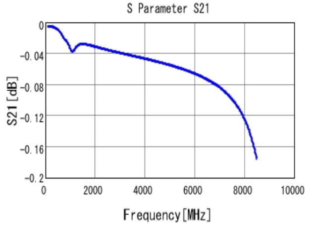
■ GRM0335C1E821JA01 S21 DCOV, 25degC
