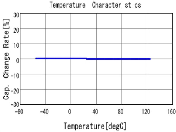
■ GRM0335C1E821JA01 C-Temp. capchange, DCOV, AC1Vrms
