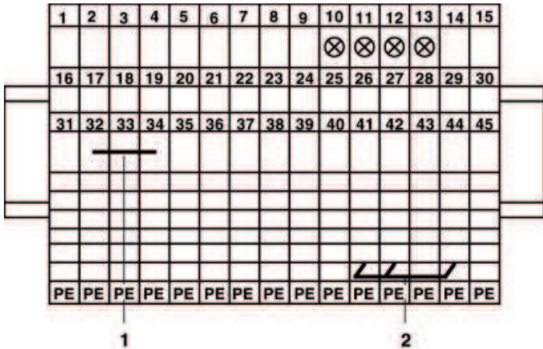
Circuit diagram
