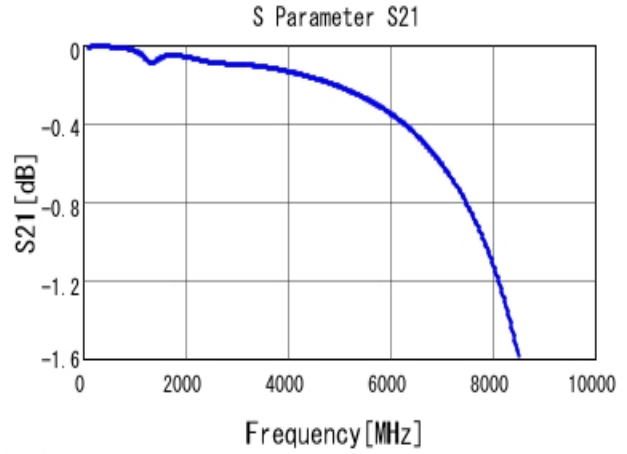
■ GCM1885C2A331JA16 S21 DCOV, 25degC
